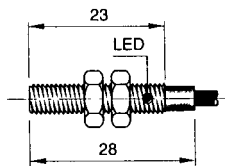
(5mm) 300-0510-XX
